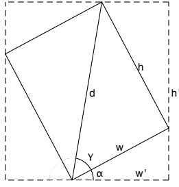
Figure 3: Rotating the patch of size h \times w by \alpha extends its bounding box (dashed lines) to new dimensions h' \times w' . Note that the length of the hypotenuse stays unchanged, while its angle to w' varies.
