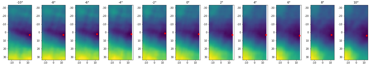
Figure 4: Slices of similarity space produced by the mean squared error between two patches in RGB color space. These patches are later shown in Figures 5a and 5b, and the merged result is shown in Figure 5d. Red dots point to the optimal displacement at each rotation. The red dot at rotation of -4^\circ marks the best overall merging location.
