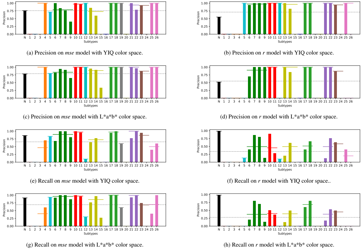
Figure 8: Evaluation of per-subtype test set classification. Lines spanning multiple bars of the same color mark supertype classification performance for each class. Dashed line indicates an average score. The color code corresponds to that in Figure 6.
